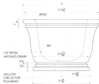
BATH TUB INTERIOR PROFILE
