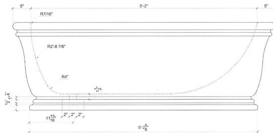
BATH TUB LONGITUDINAL INTERIOR PROFILE
